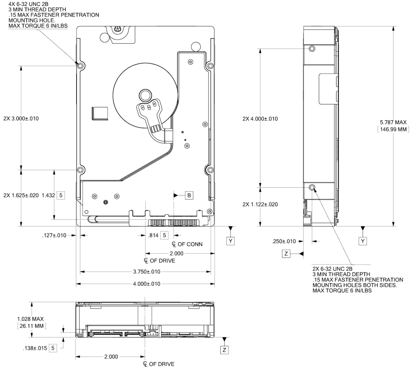
Figure 3 Mounting dimensions
