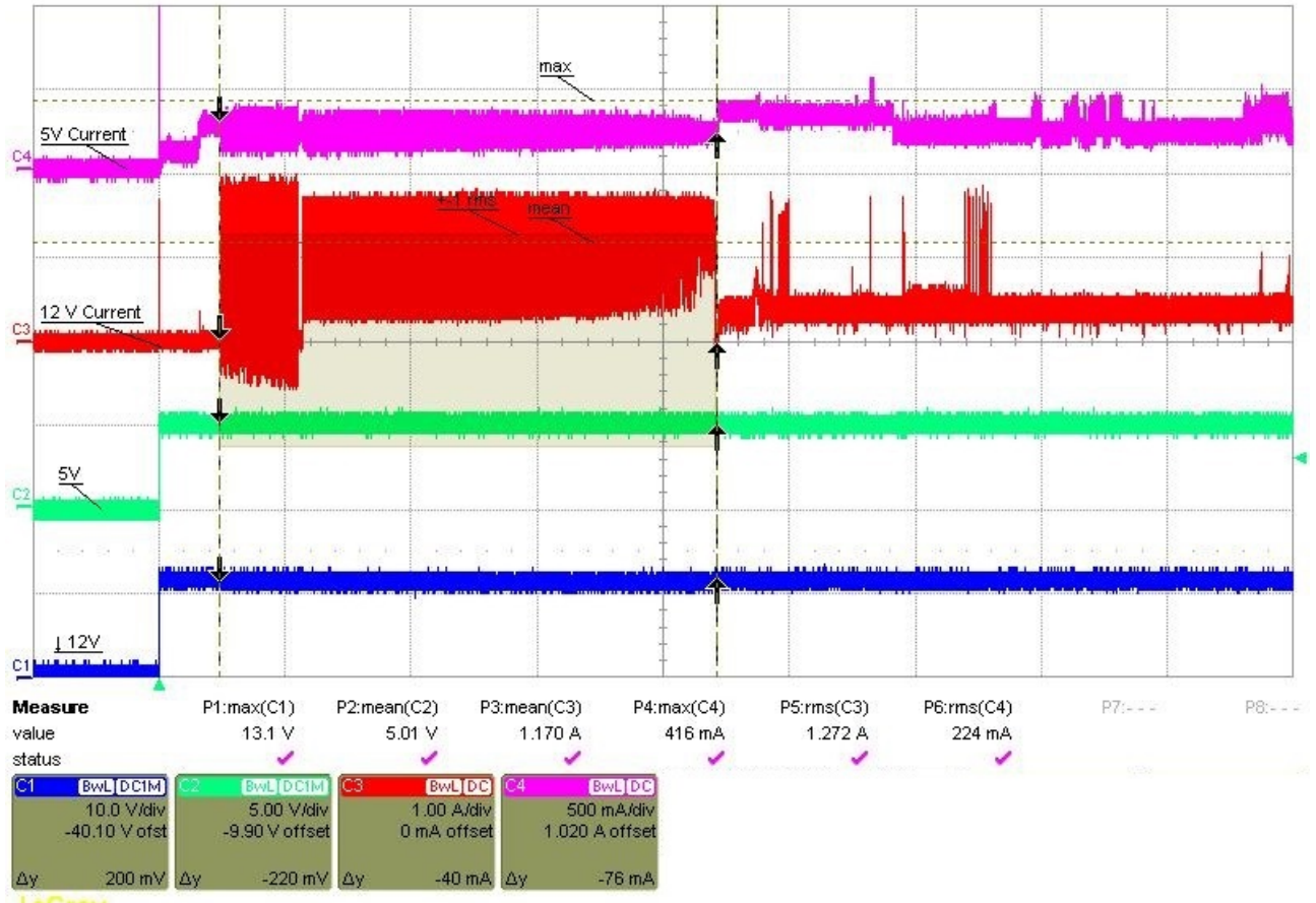
Figure 1 Typical 5TB model 5V & 12V - 6Gb/s startup and operation current profiles
