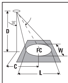
Candlepower Distribution 20W Lamp t4.5 – Spot Upper Reflector
